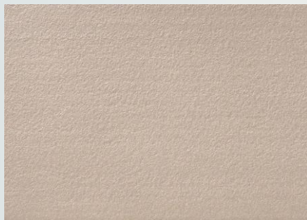
Iceberg
